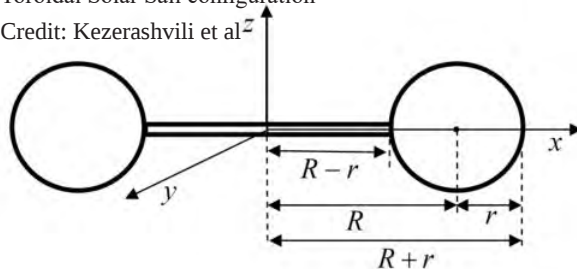
Toroidal Solar Sail configuration
